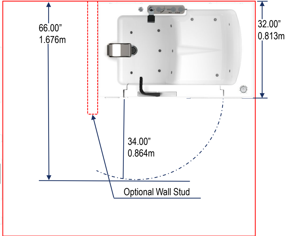
End Wall Installation
